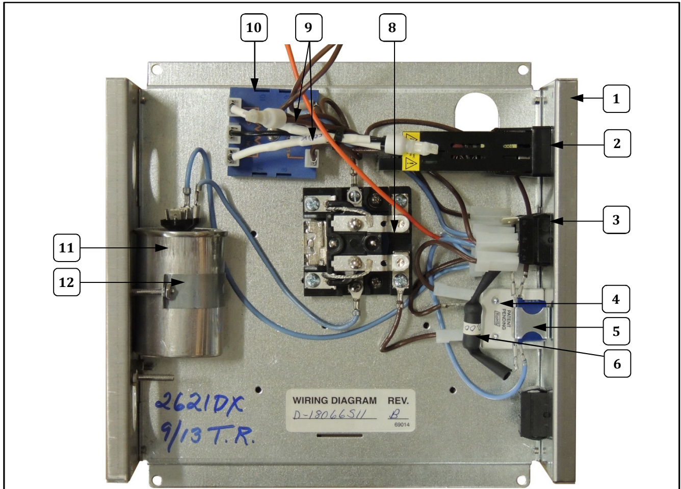
Digital Control Panel Interior View (Model 2621DX Shown)
